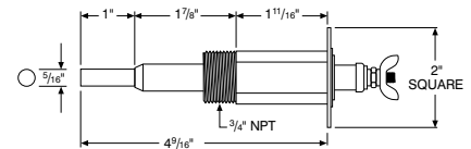
EL1214-P – 3/4" NPT
