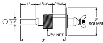
EL1214-SV - 3/4" NPT For 1/2", order No. EL1220-SV
