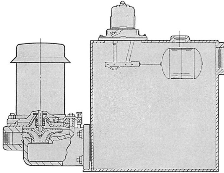
TYPICAL VMX CROSS-SECTION
