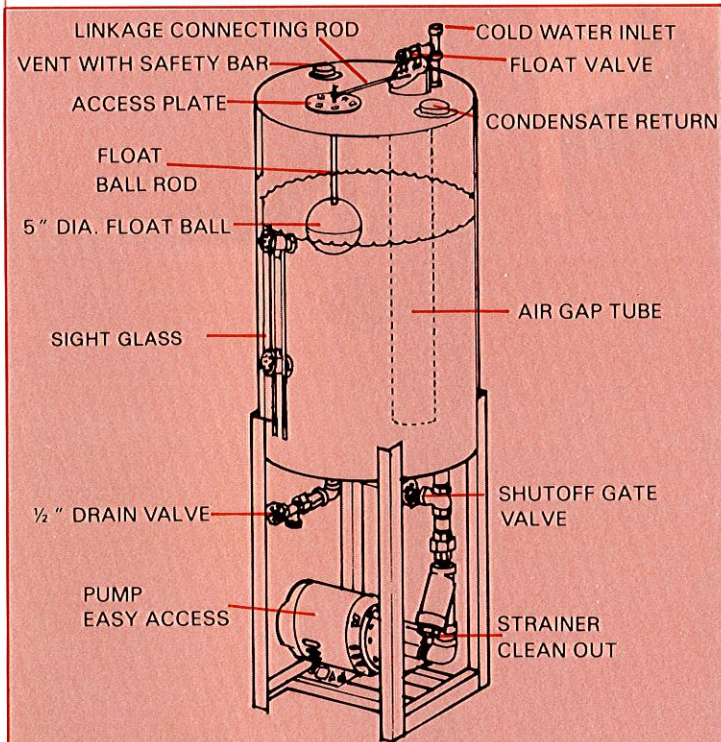
VERTICAL Return System with Burks Pump
