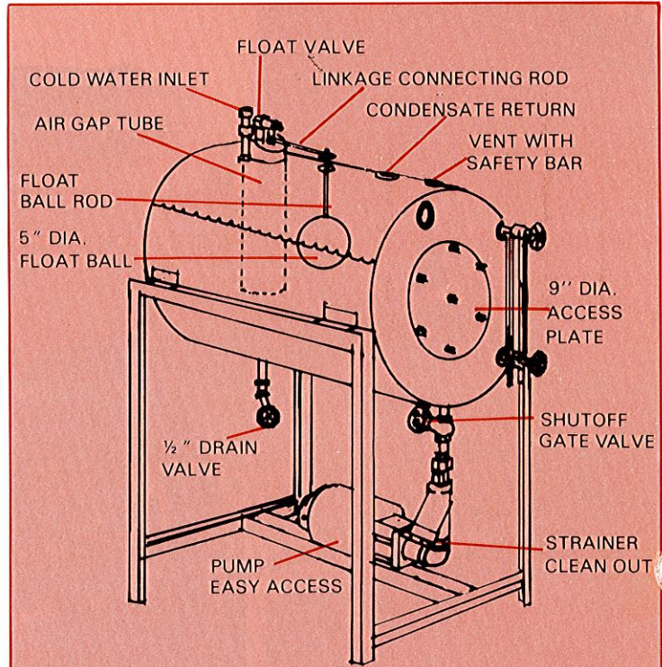
HORIZONTAL Return System with Burks Pump
