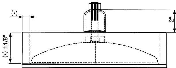
MANHOLE ASSM FRONT VIEW
